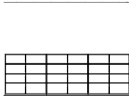
2 18.13 BOOKSHELF ELEVATION AS9-1813 SCALE 1:30
