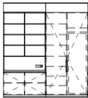
2 18.03 JOINERY ELEVATION A90-1802 SCALE 1:50
