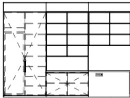
2 18.06 JOINERY ELEVATION SCALE: 1:50
