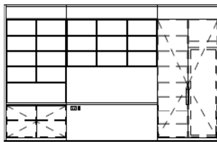
2 18.04 JOINERY ELEVATION SCALE 1:50
