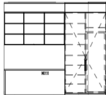
3 18.13 DESK ELEVATION AS9-1813 SCALE 1:30
