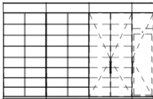
2 18.11 JOINERY ELEVATION SCALE: 1:30
